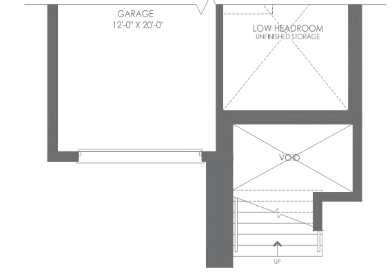
PARTIAL STANDARD & OPTIONAL GROUND FLOOR ELEV. B
