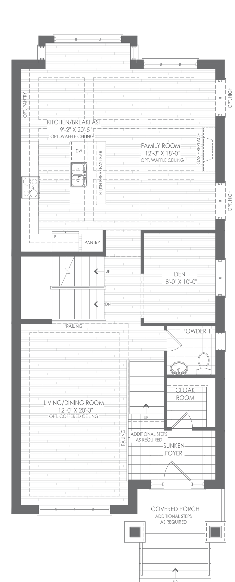
SECOND FLOOR ELEV. A (MAIN LIVING/KITCHEN LEVEL)
