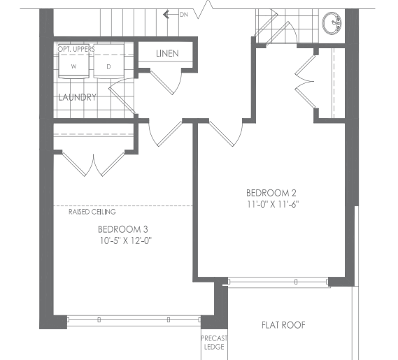
PARTIAL STANDARD AND OPTIONAL THIRD FLOOR ELEV. B
