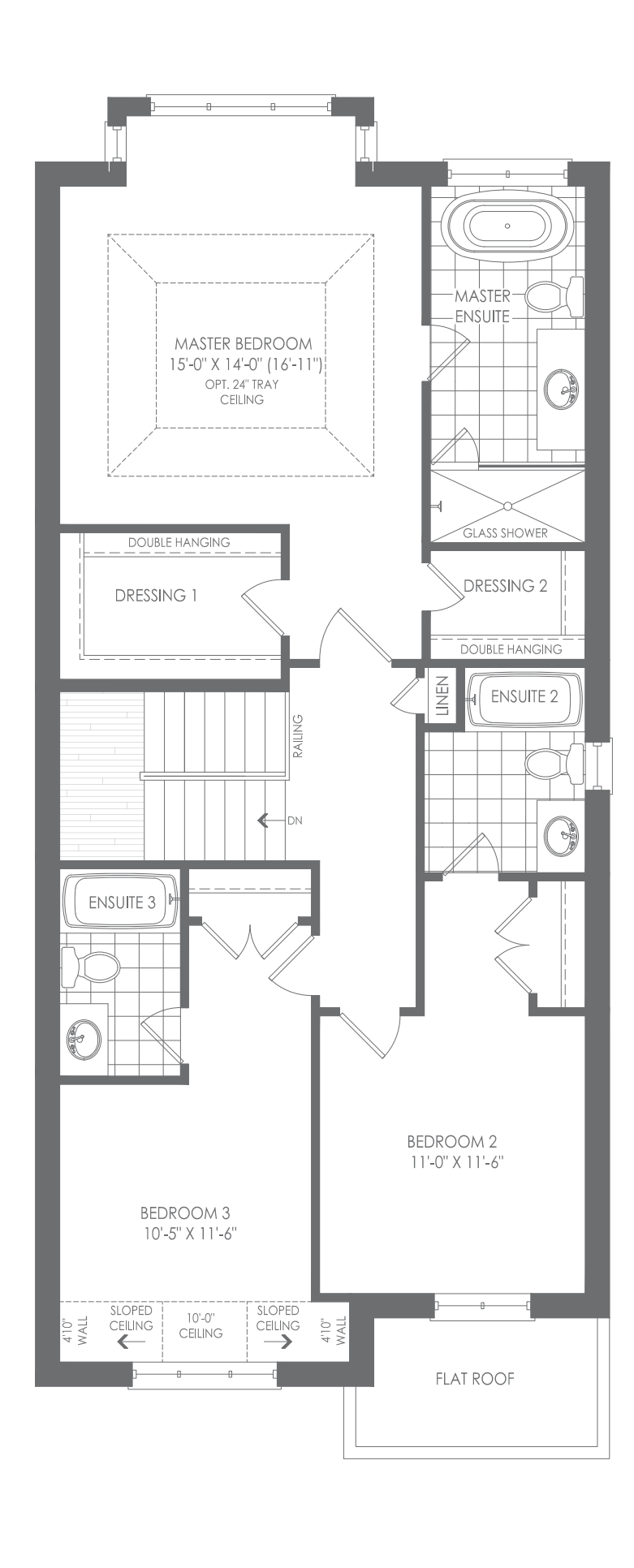
OPTIONAL THIRD FLOOR ELEV. A THIRD BATH FLEX PLAN WITH GROUND FLOOR LAUNDRY
